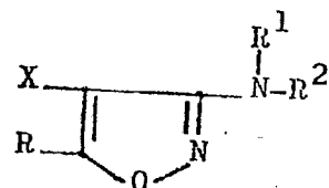
(I-g: R 2 =Acyl)
